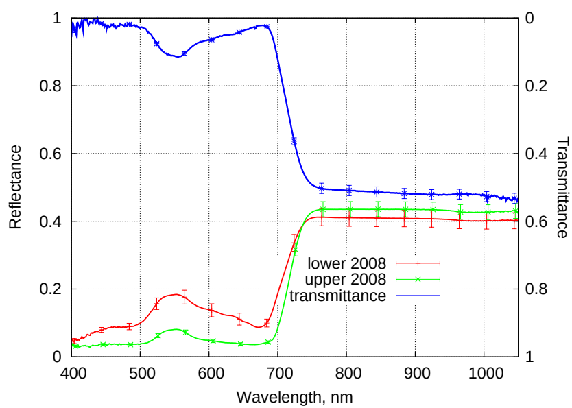
Figure 6.20: Leaf reflectance and transmittance of Populus tremula .
